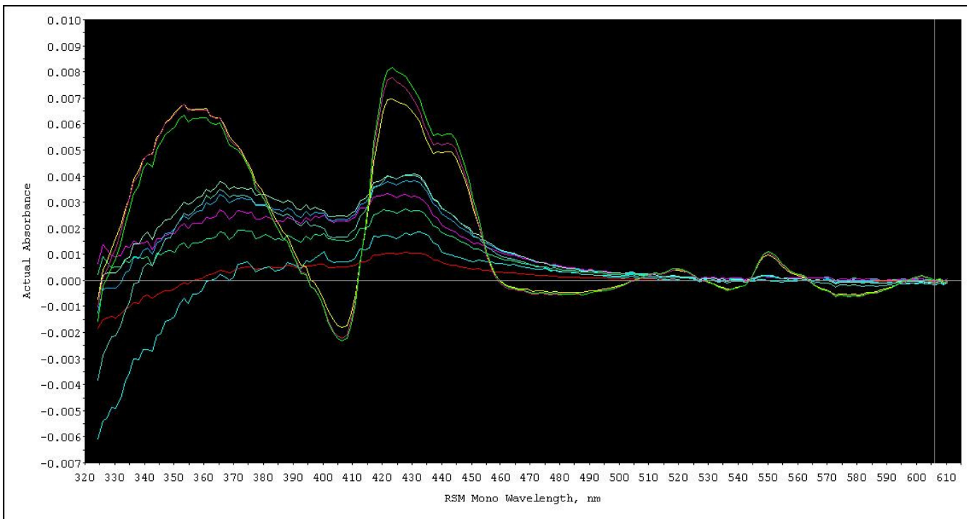
Difference spectra
